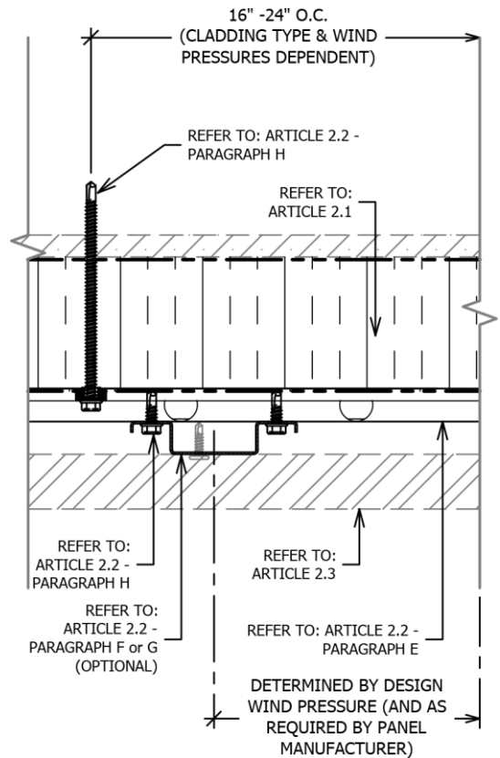
PLAN VIEW
