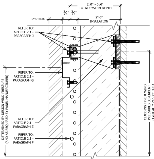
SECTION VIEW
